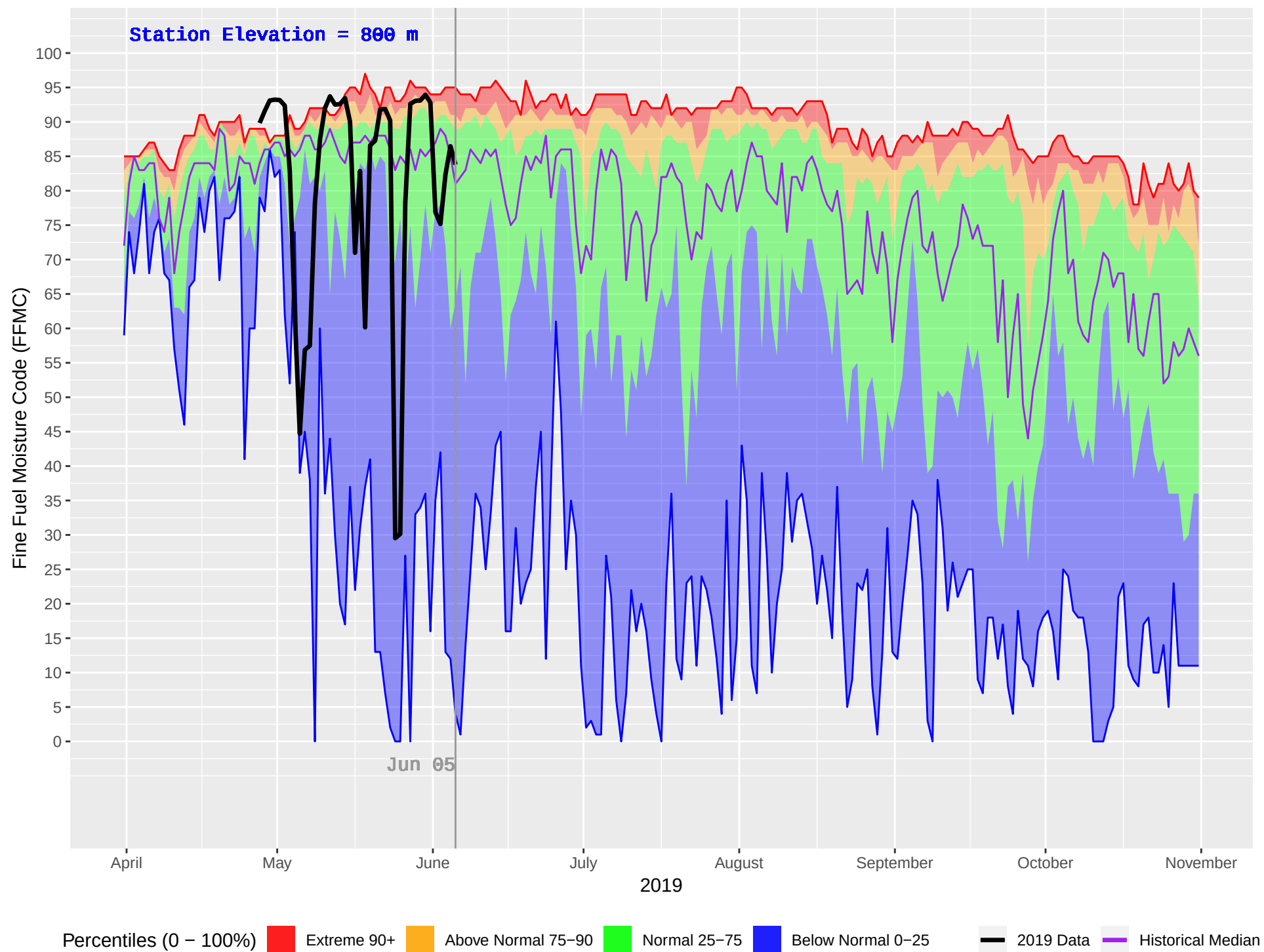
DEASE LAKE FS (108) : Historical (1978–2018) and Current (2019) Daily Fine Fuel Moisture Code (FFMC)
