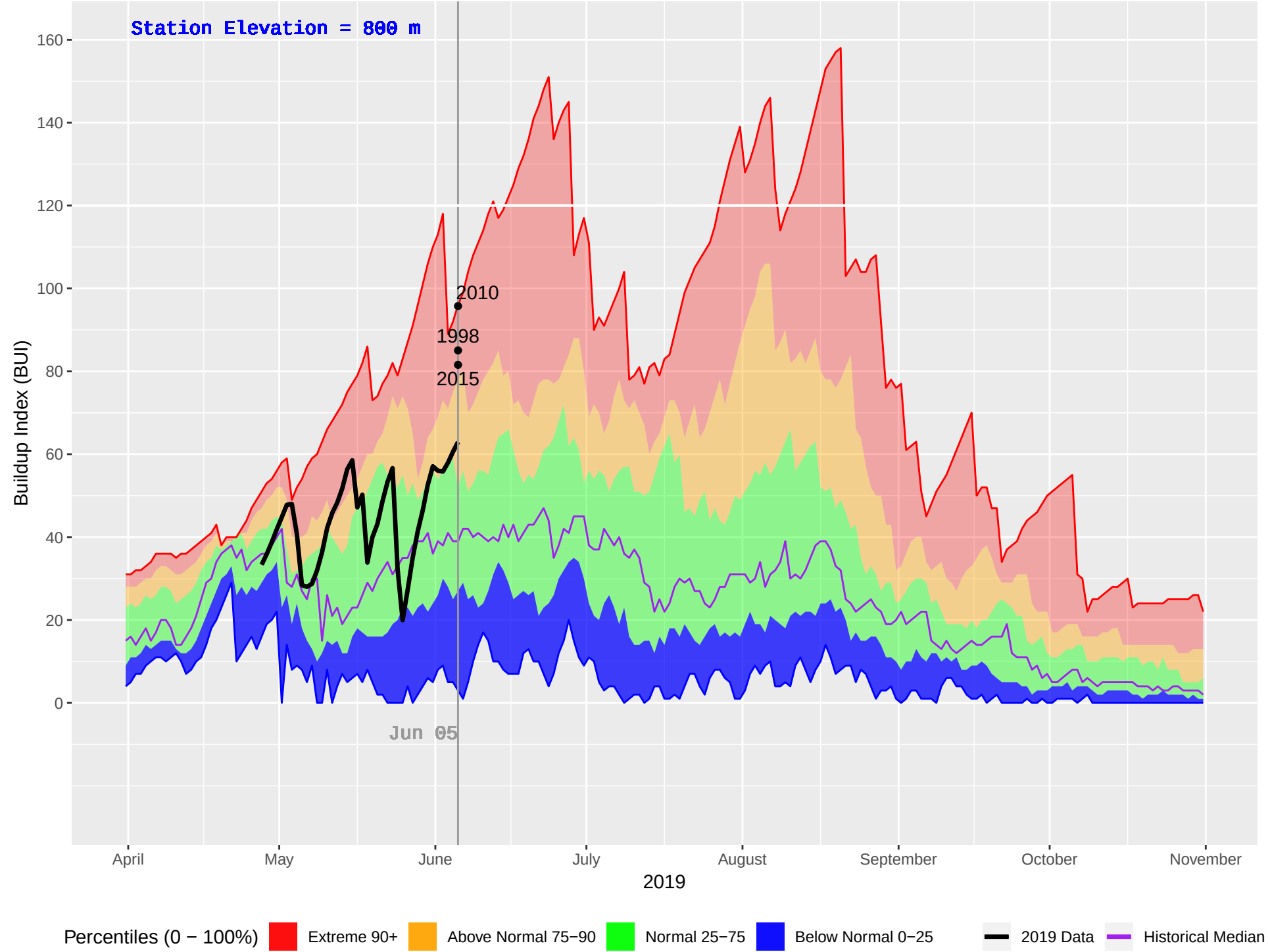
DEASE LAKE FS (108) : Historical (1978–2018), Current (2019) Daily Buildup Index (BUI)
