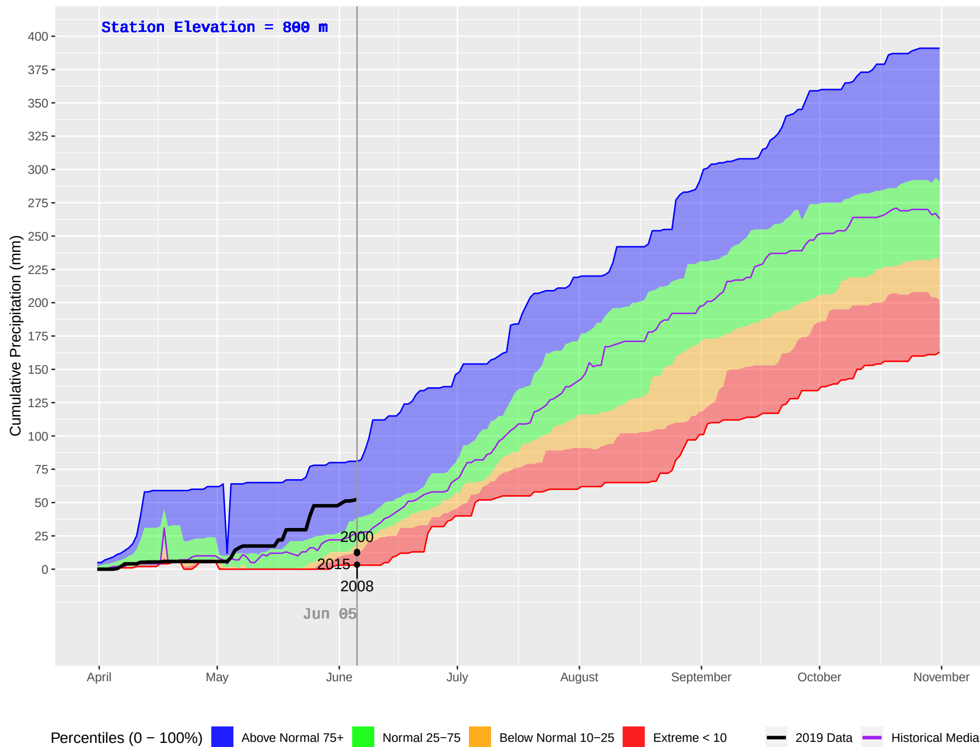
DEASE LAKE FS (108) : Historical (1978–2018), Current (2019) Daily Cumulative Precipitation
