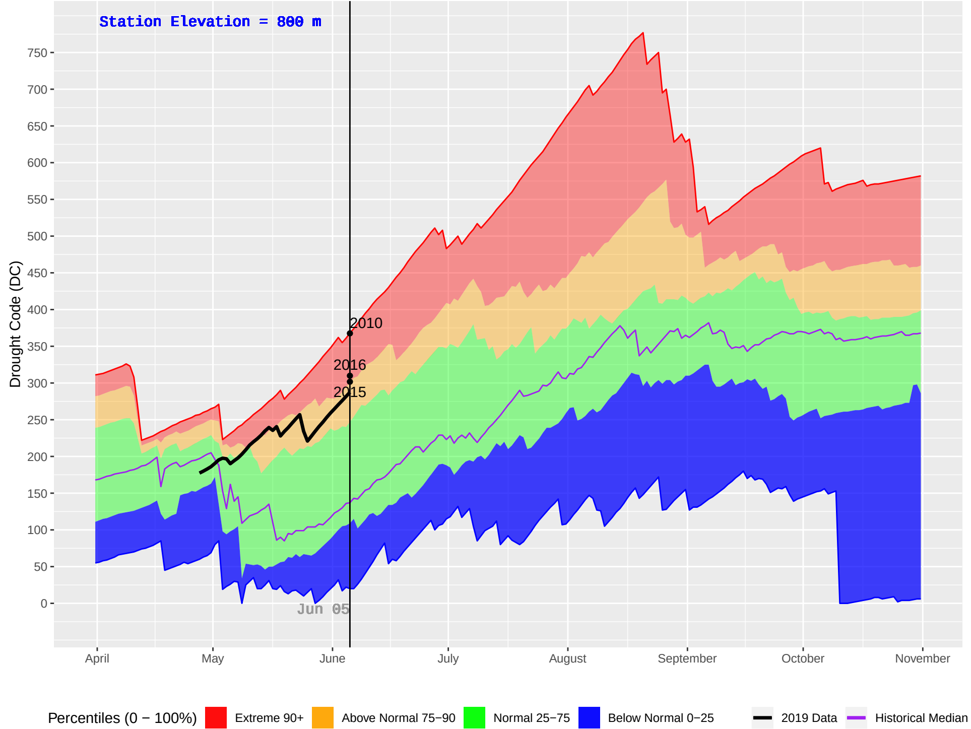
DEASE LAKE FS (108) : Historical (1978–2018) and Current (2019) Daily Drought Code (DC)
