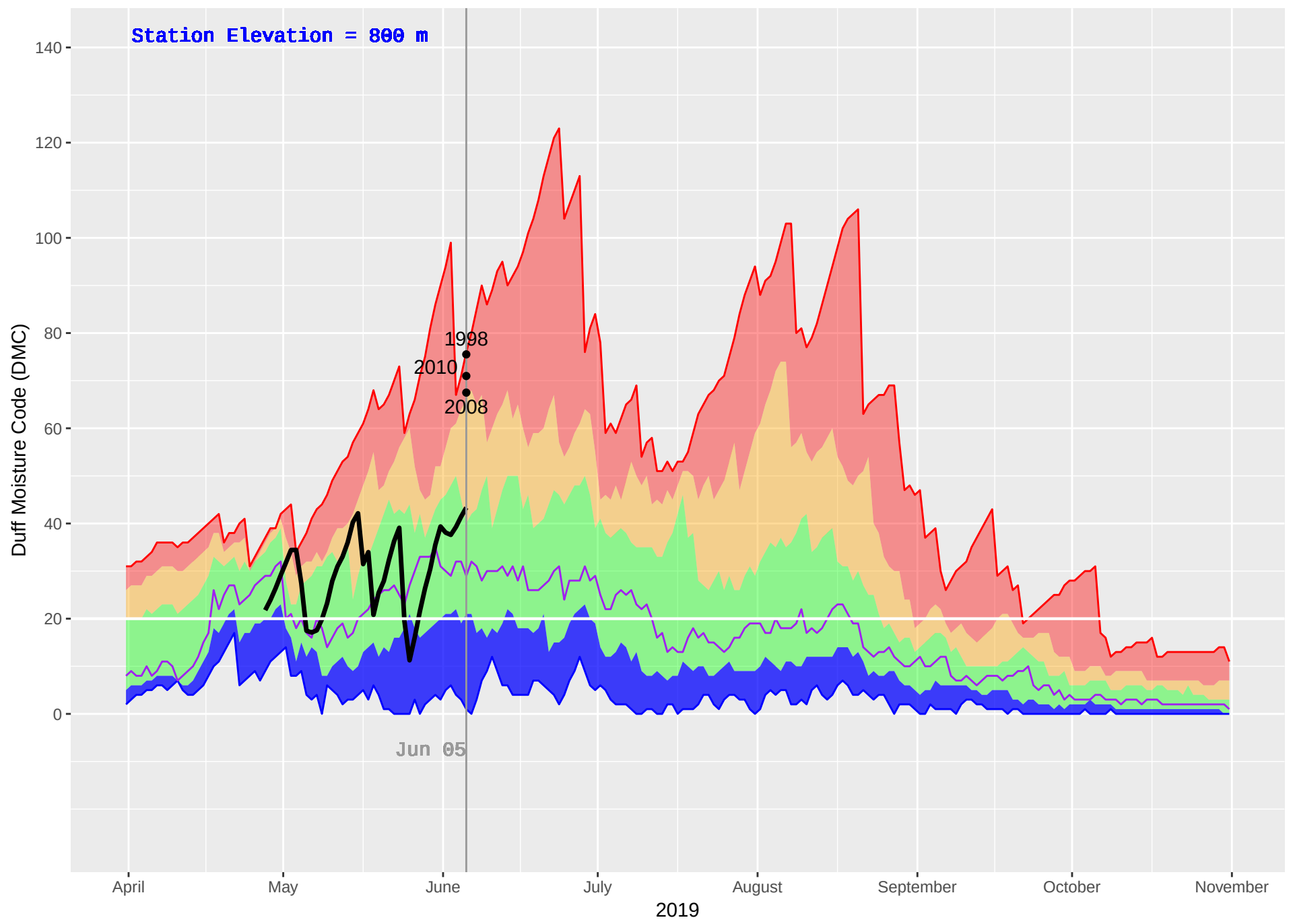
DEASE LAKE FS (108) : Historical (1978–2018), Current (2019) Daily Duff Moisture Code (DMC)
