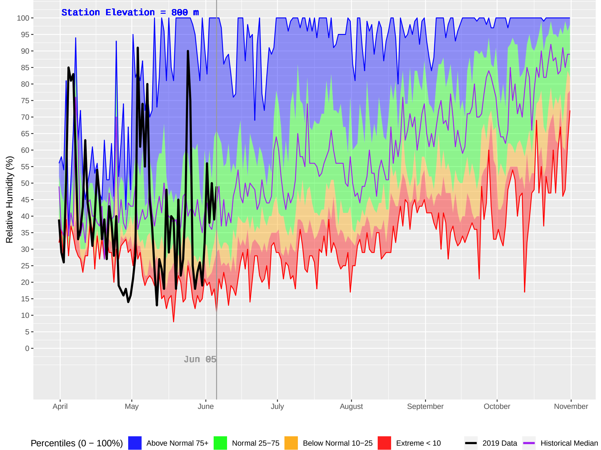
DEASE LAKE FS (108) : Historical (1978–2018) and Current (2019) Daily Relative Humidity
